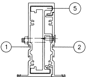
MULLION 'M2'
