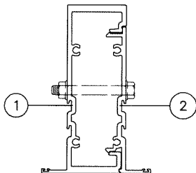
MULLION 'M1'
