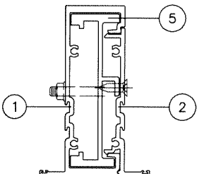
MULLION 'M2'
